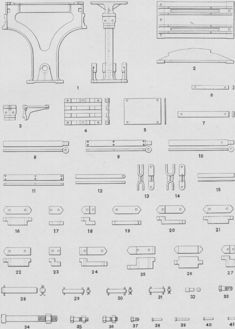
LEGS, TOP PLATES, BEARINGS, LOCKING PLATES, ETC., FOR FOR STEVENS INTERLOCKING MACHINE
